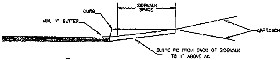
- CURB SECTION -
