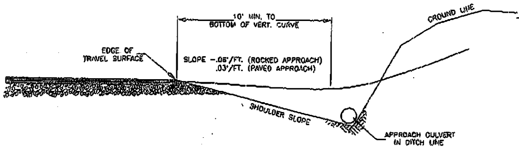
- CUT SECTION -
